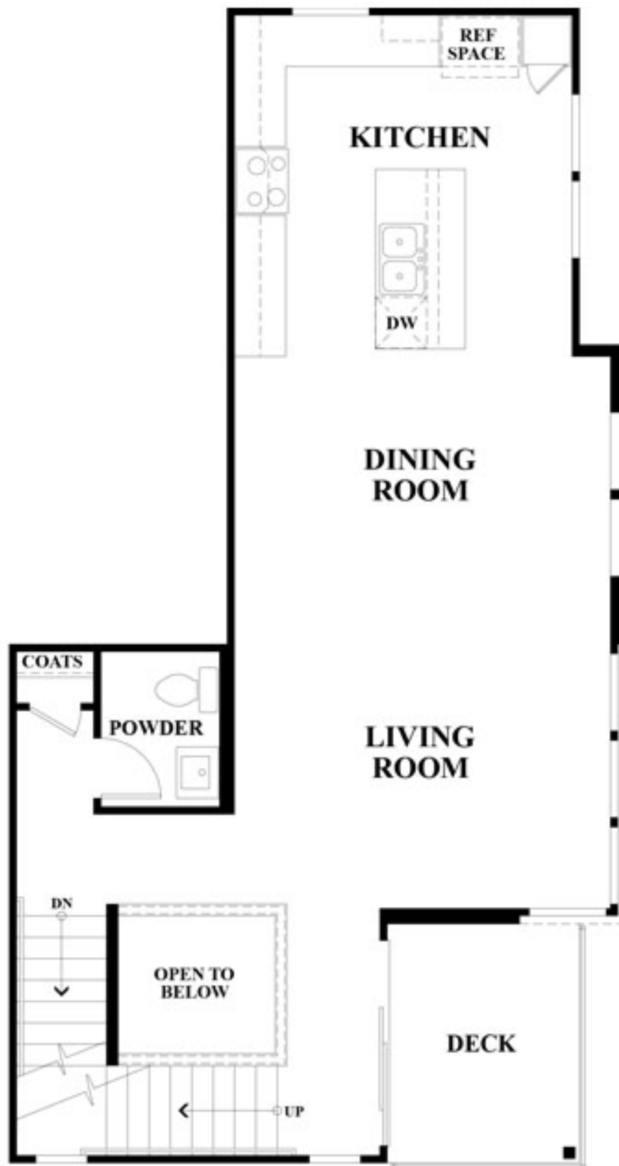
PLAN 4 SECOND FLOOR
